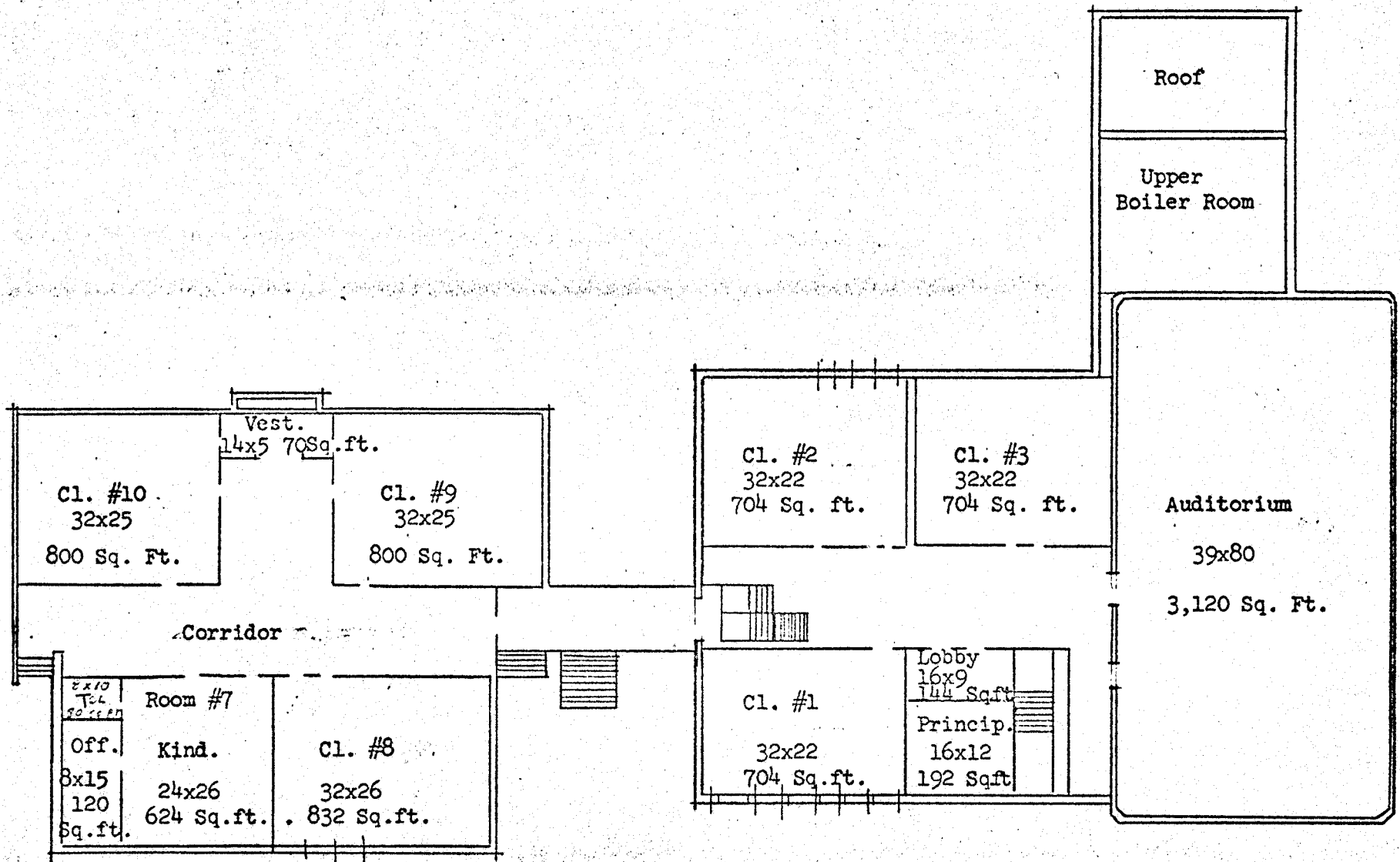
CAMP SCHOOL FIRST FLOOR.
