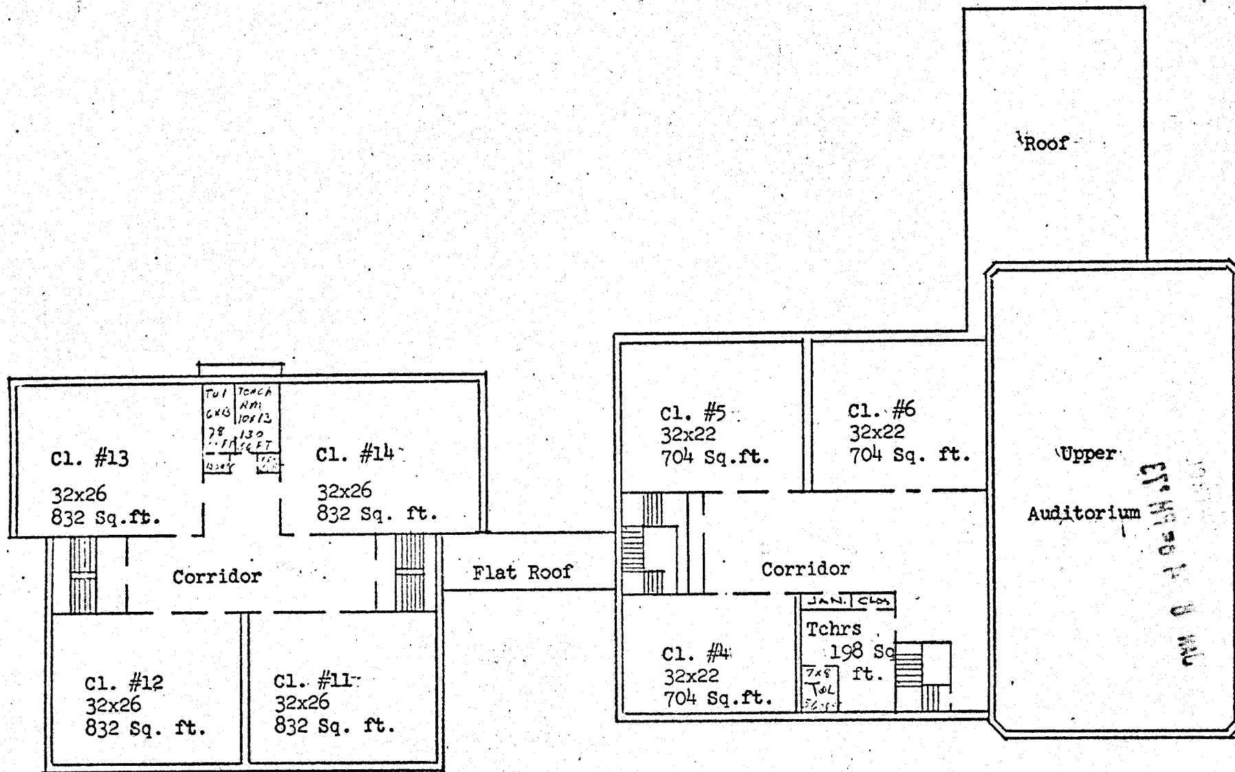
CAMP SCHOOL SECOND FLOOR
